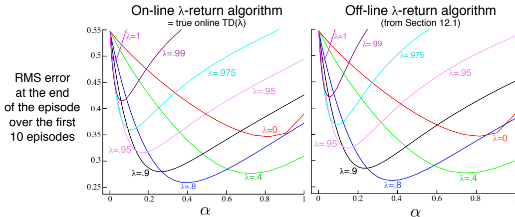
Figure 12.8: 19-state Random walk results (Example 7.1): Performance of online and off-line \lambda -return algorithms. The performance measure here is the \overline{\text{VE}} at the end of the episode, which should be the best case for the off-line algorithm. Nevertheless, the online algorithm performs subtly better. For comparison, the \lambda=0 line is the same for both methods.
