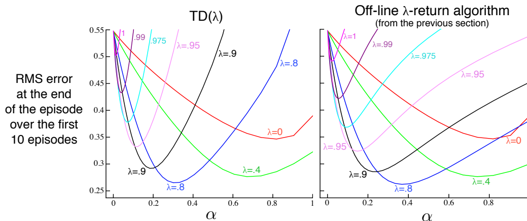
Figure 12.6: 19-state Random walk results (Example 7.1): Performance of \text{TD}(\lambda) alongside that of the off-line \lambda -return algorithm. The two algorithms performed virtually identically at low (less than optimal) \alpha values, but \text{TD}(\lambda) was worse at high \alpha values.
